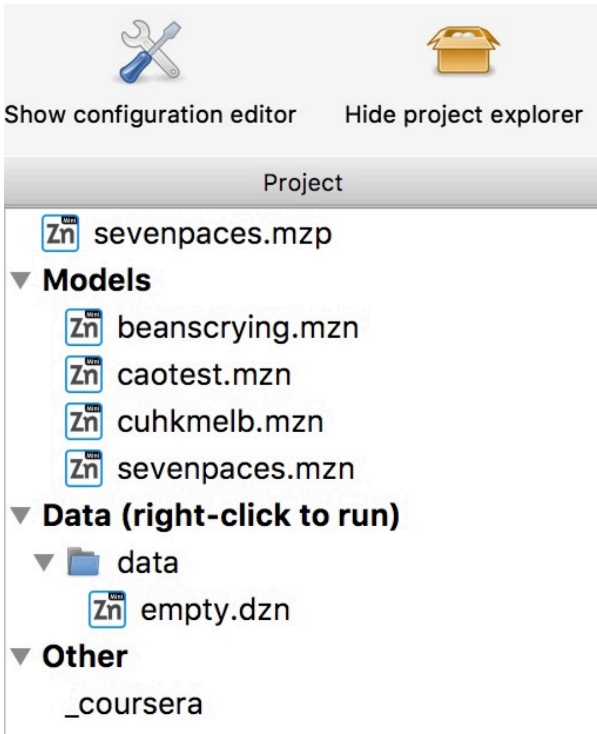
Fig. 3.2.3: Project explorer
